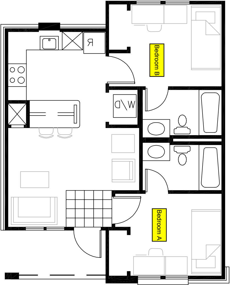
EAST CAMPUS APARTMENTS 2 BEDROOM SCALE: 3/16" = 1'-0"
